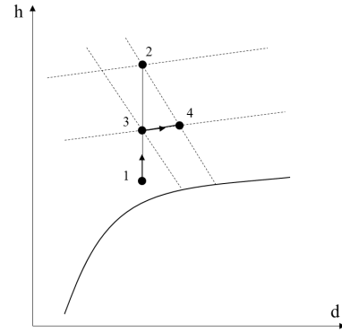
Figure 8 Enthalpy wet figure of the heating processes of the cooling air
