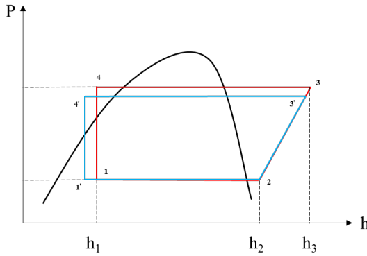
Figure 7 Refrigeration cycle comparison before and after adding spray
