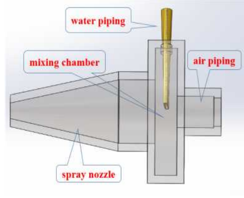
Figure 6 schematic diagram of spray nozzle
