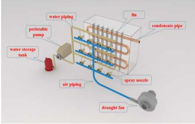
Figure 5 the overall system diagram
